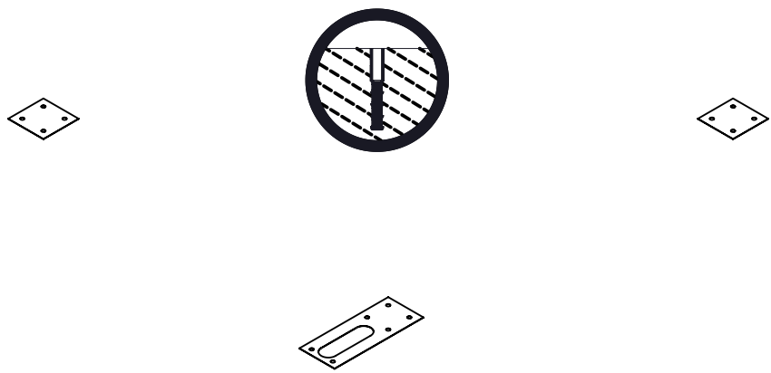
POST ANCHORS' INSTALLATION REFER TO ANCHORING MARKING METHOD ON P. TYP - 01 REFER TO ANCHOR ASSEMBLY DETAIL ON P. TYP - 02 USE INSTALLATION DRAWING MEASUREMENTS FOR MORE DETAILS
