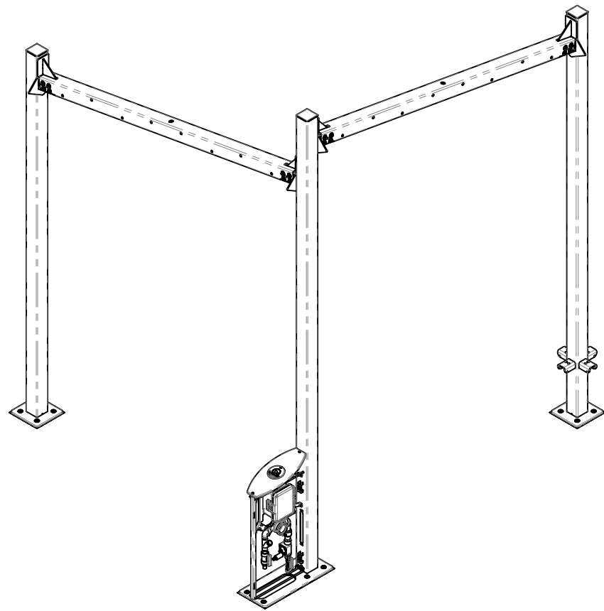
BEAMS INSTALLATION FULLY SECURE THE POSTS WITH TOOLS AFTER ALL BEAMS ARE INSTALLED REFER TO BEAM ASSEMBLY DETAIL ON P. TYP - 07
