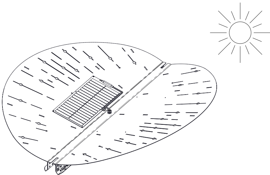
CANOPIES WITH SOLAR PANEL ORIENTATION CANOPIES WITH SOLAR PANEL MUST BE INSTALLED TOWARDS THE SUN (SOLAR PANEL FACING SOUTH IN NORTH HEMISPHERE / FACING NORTH IN SOUTH HEMISPHERE) AVOID SHADOW AND OBSTRUCTED AREAS REFER TO CANOPY ASSEMBLY DETAIL ON P. TYP - 09
