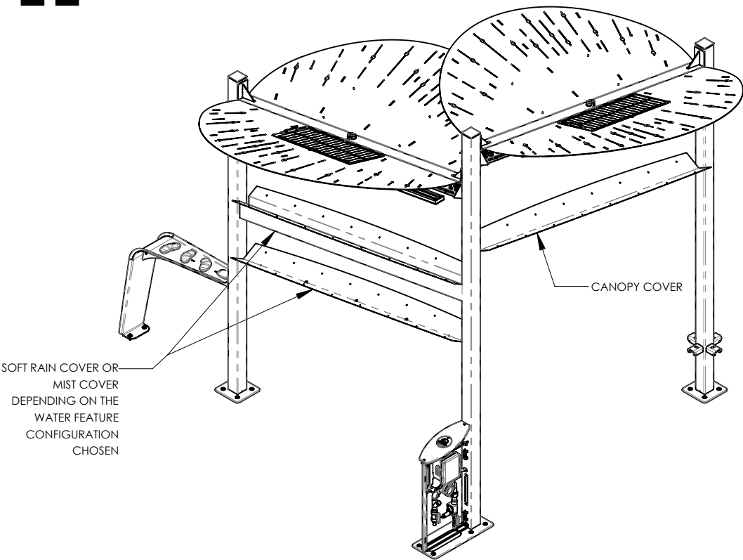
COVERS INSTALLATION COVER TYPE MAY VARY DEPENDING ON WATER FEATURE REFER TO COVER ASSEMBLY DETAIL ON P. TYP - 23
