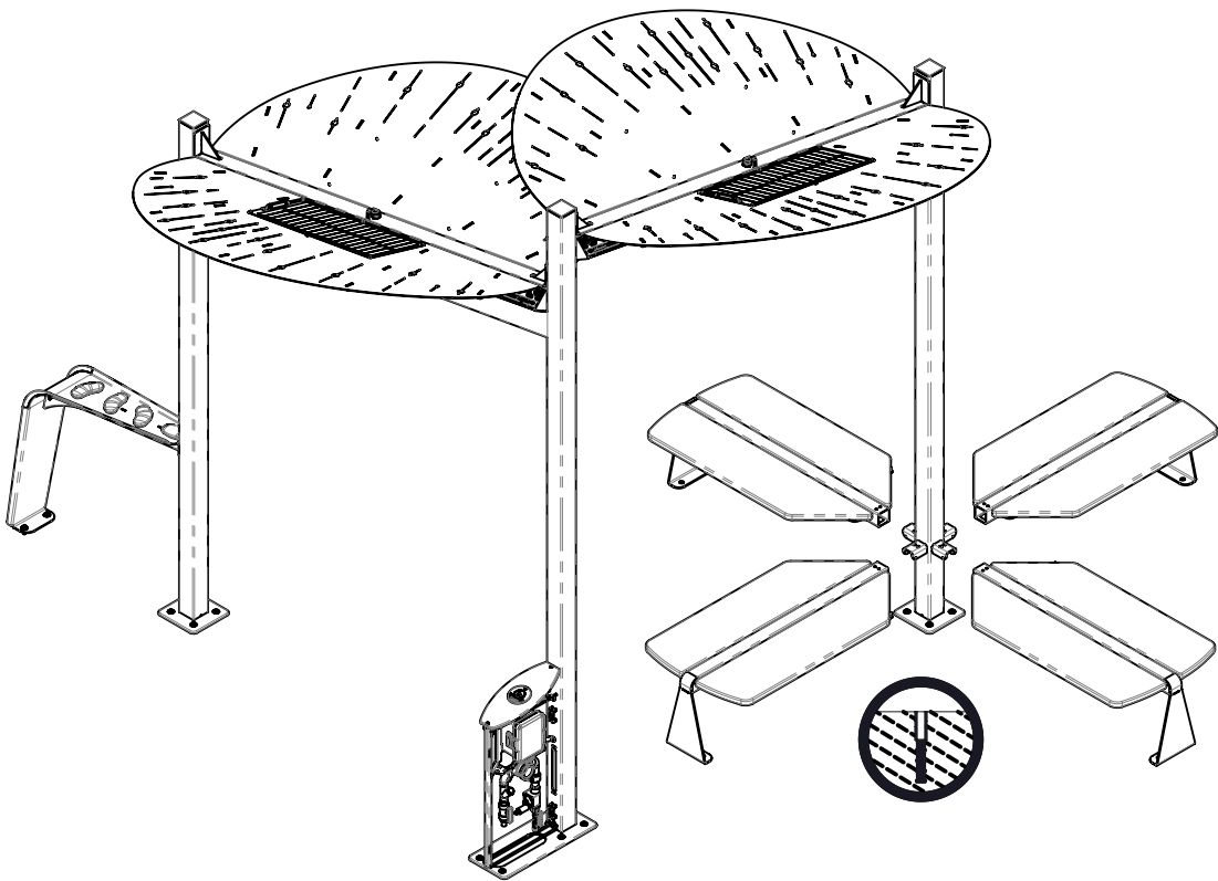
BENCHES INSTALLATION REFER TO BENCH WITH BACKREST SEATING ASSEMBLY DETAIL ON P. TYP - 24 REFER TO BENCH FLAT SEATING ASSEMBLY DETAIL P. TYP - 28
