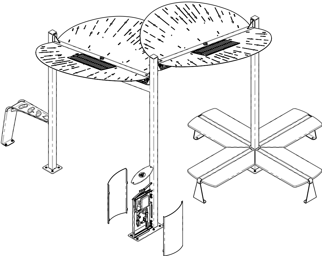
WMS SIDE PANELS INSTALLATION REMOVE ACTIVATOR PLATE TO INSTALL THE WMS SIDE PANELS REFER TO WMS POST ASSEMBLY DETAIL ON P. TYP - 05
