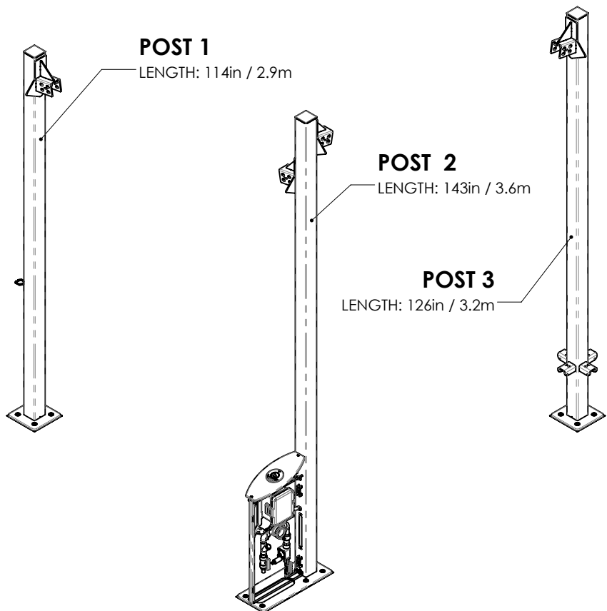
POSTS INSTALLATION HAND-TIGHTEN THE POSTS ON THE GROUND REFER TO WMS POST ASSEMBLY DETAIL ON P. TYP - 03 REFER TO POST ASSEMBLY DETAIL ON P. TYP - 06
