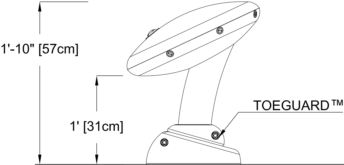
FRONT ELEVATION VIEW
