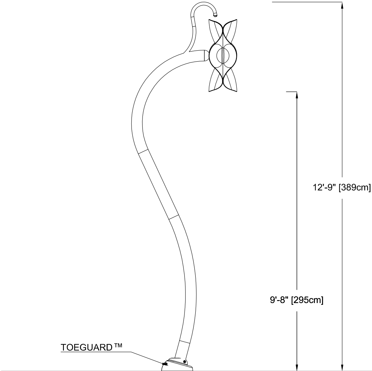
FRONT ELEVATION VIEW
