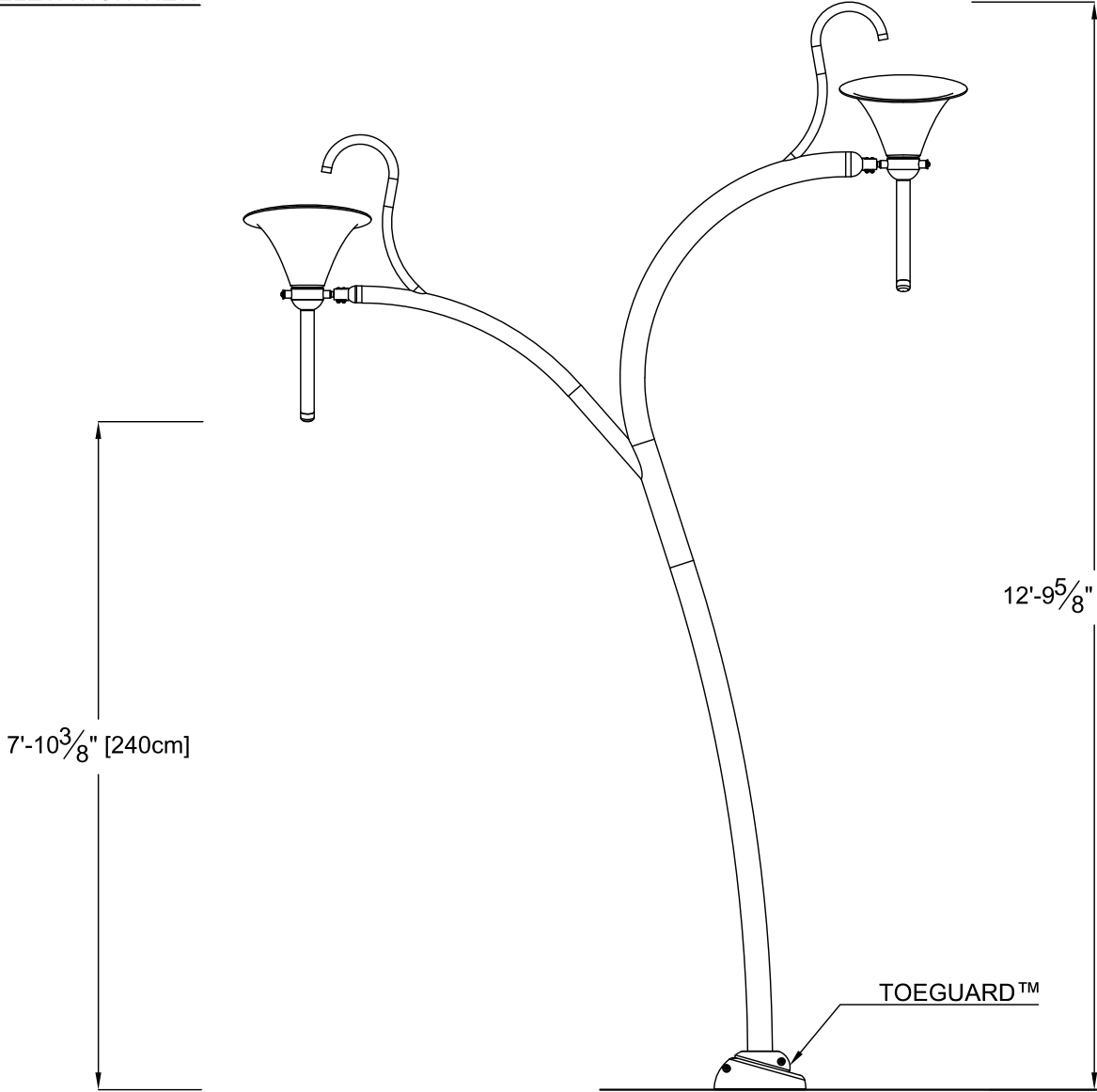
FRONT ELEVATION VIEW
