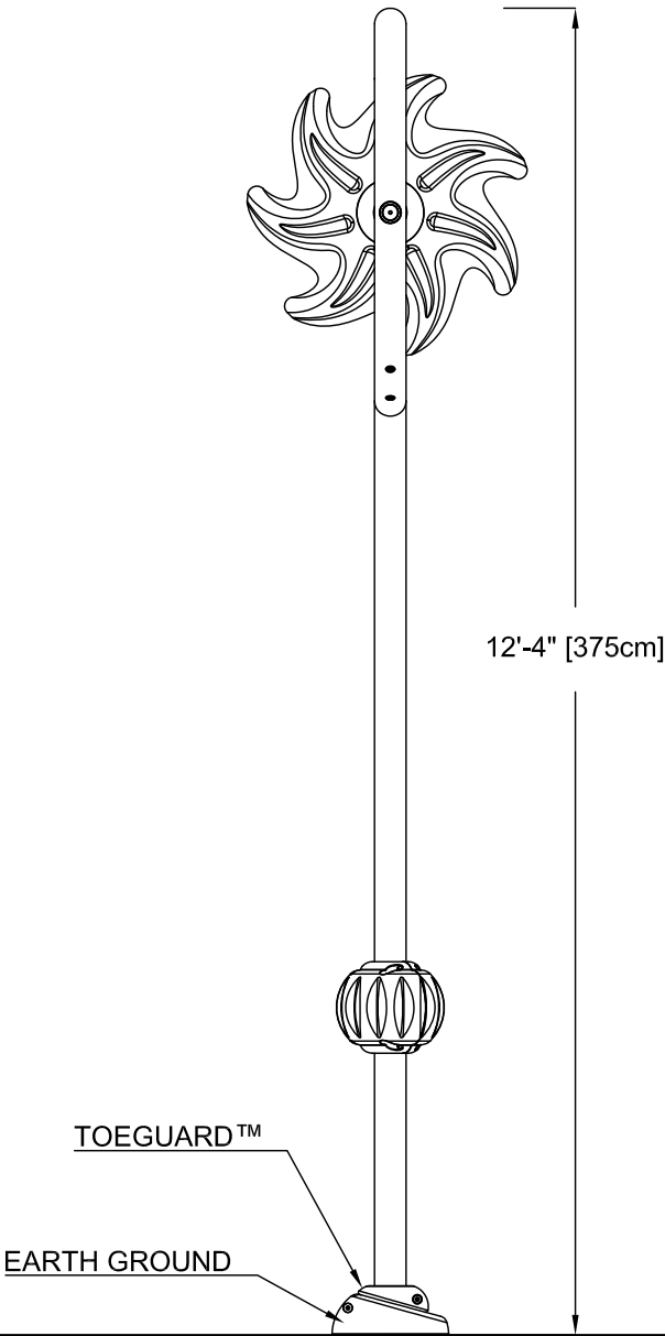
FRONT ELEVATION VIEW
