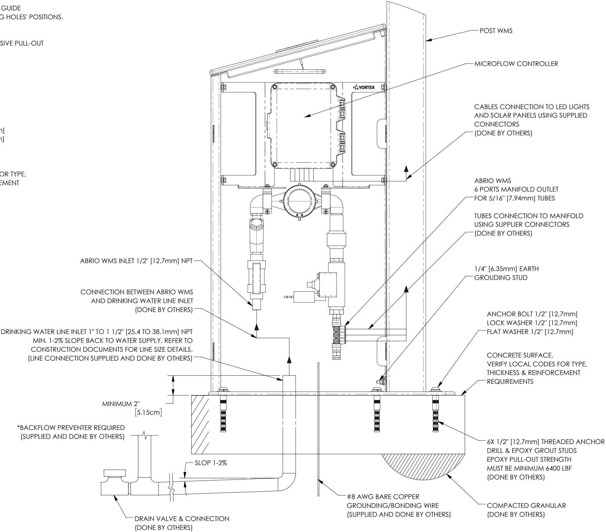
POST WMS TYPICAL ANCHORING DETAIL
