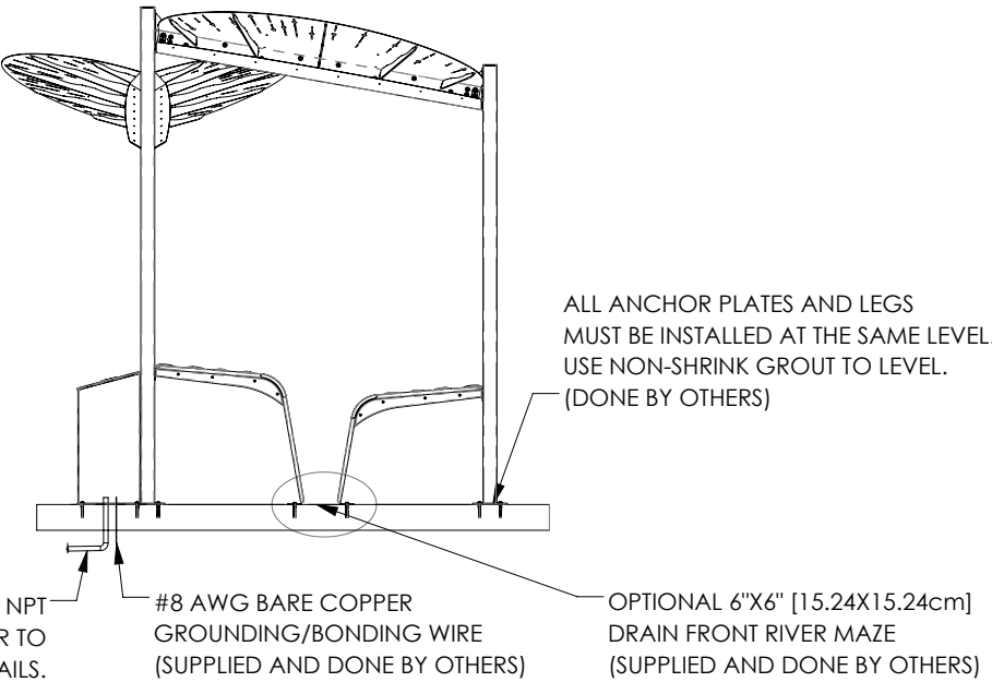
SIDE ELEVATION VIEW
