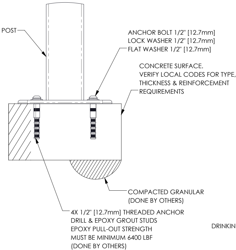
POST TYPICAL ANCHORING DETAIL
