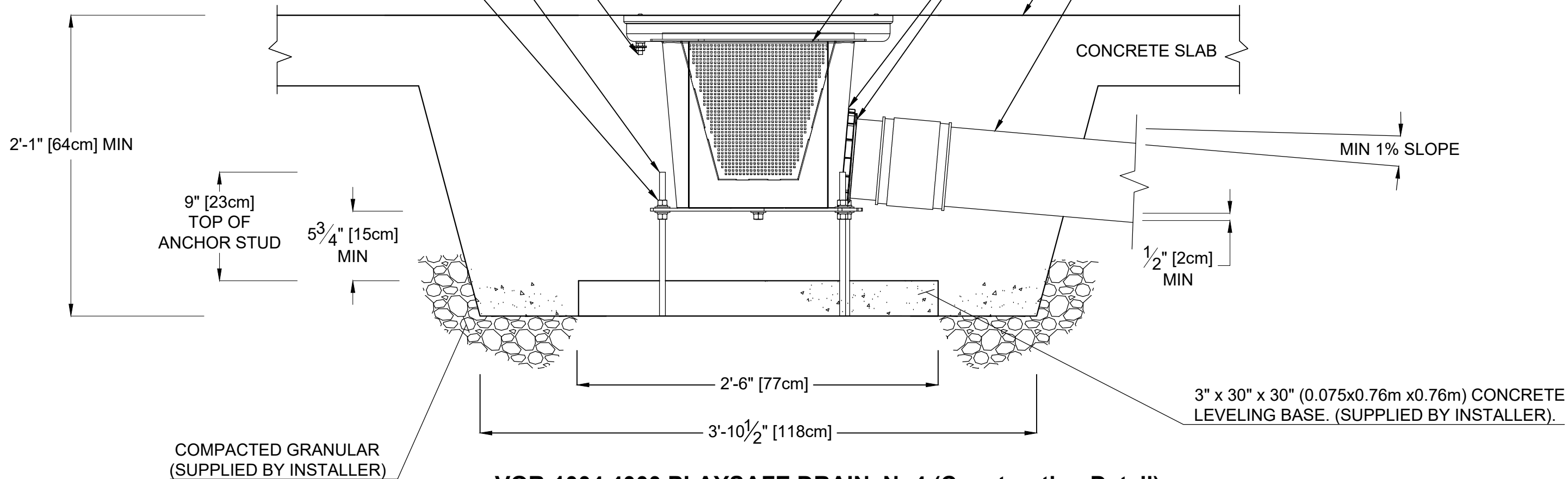
VOR-1004.4000 PLAYSAFE DRAIN, No4 (Construction Detail)
