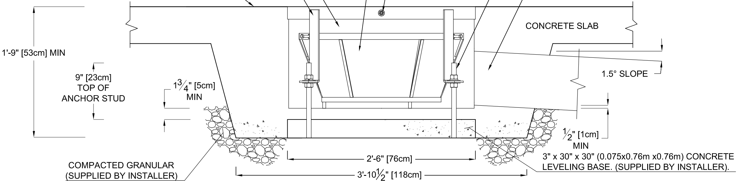
VOR-1001.4000 PLAYSAFE DRAIN, No1 (Construction Detail)
