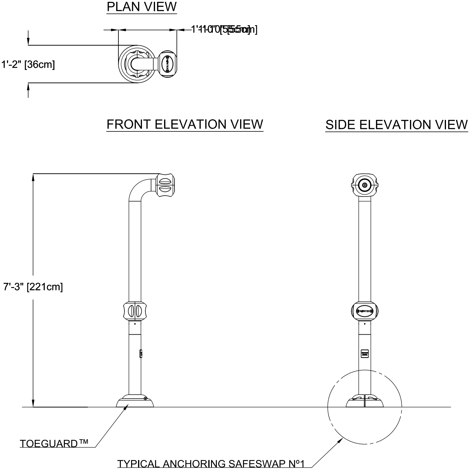
VOR-0533.2XXX PERISPRAY (Construction Detail)
