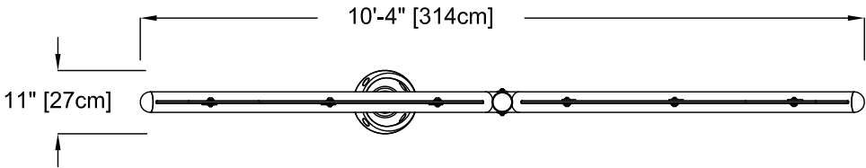
PLAN VIEW
