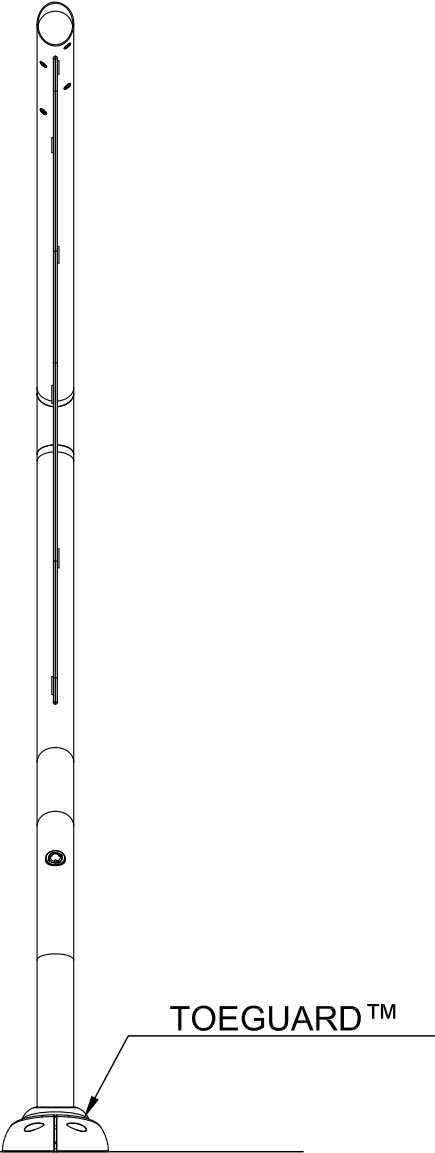
SIDE ELEVATION VIEW
