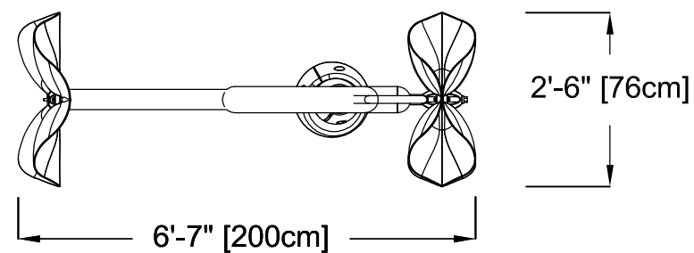
FRONT ELEVATION VIEW
