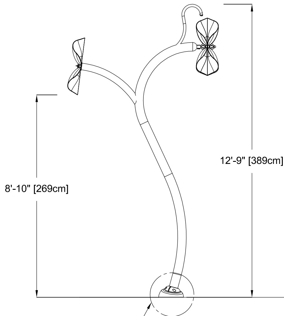
FRONT ELEVATION VIEW
